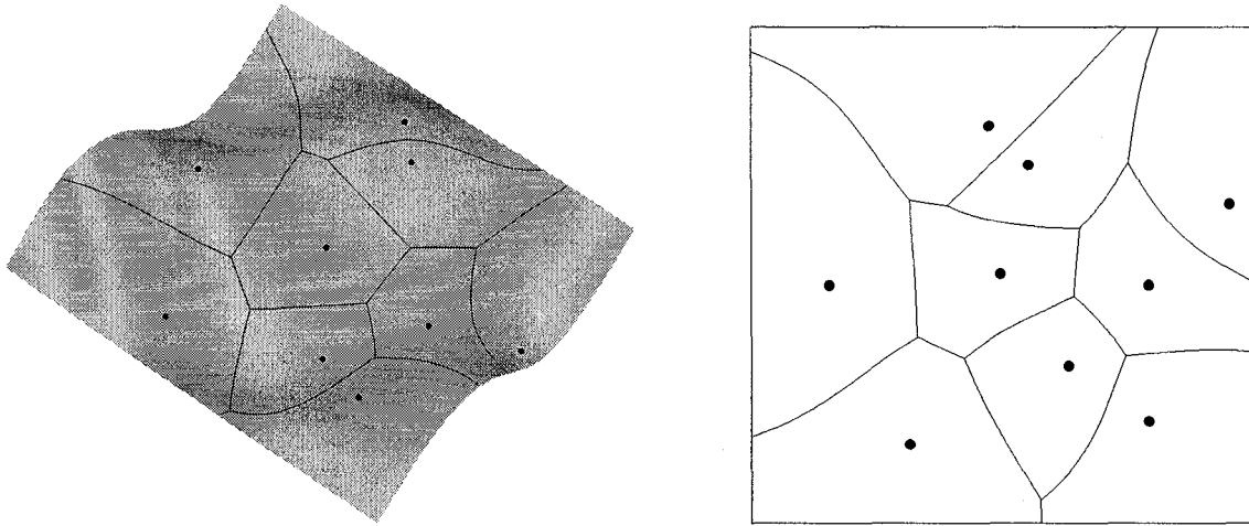
Figure 3. Voronoi diagram on a wave-like surface and corresponding curves in parameter space
