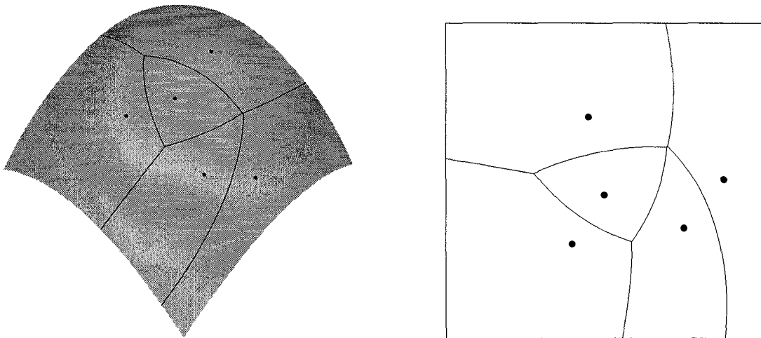
Figure 4. Voronoi diagram on a paraboloid and corresponding curves in parameter space
